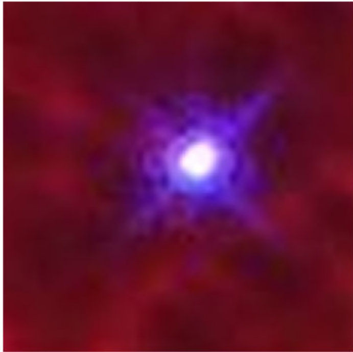
Spline method
