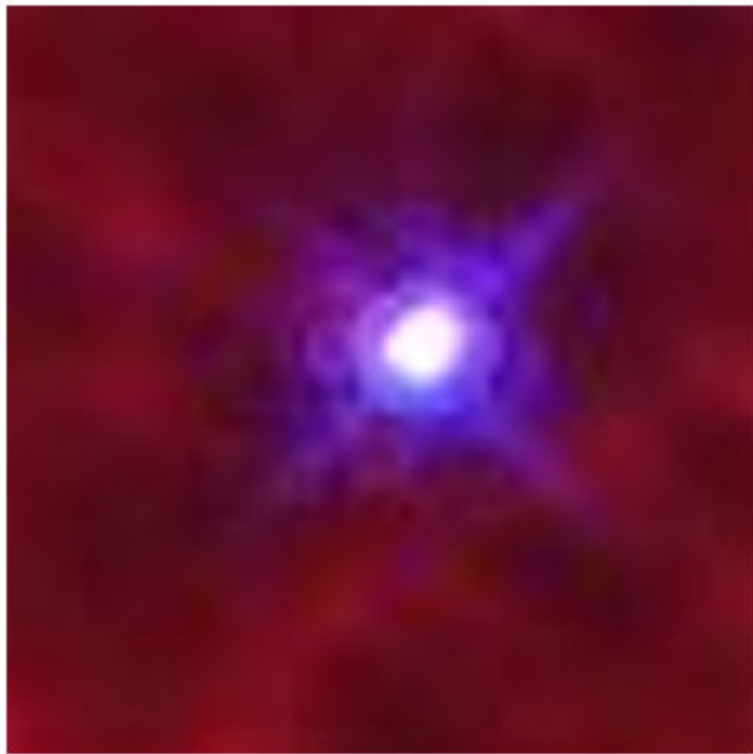
Cubic method
